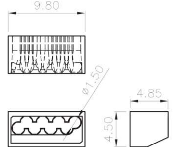
SCALE 5/1
